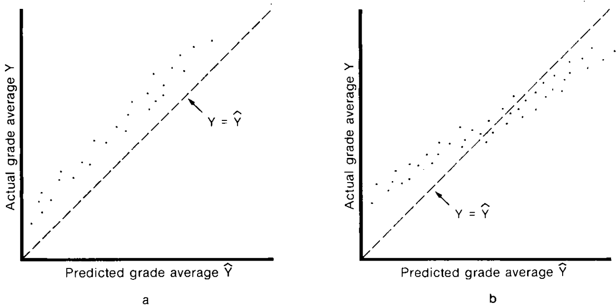
Figure 1. Two situations in which cross-validated r gives a false indication of prediction quality
